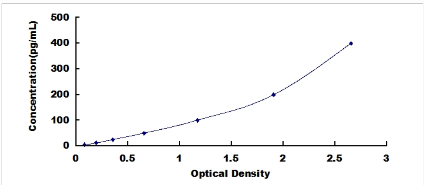
Typical Standard Curve for Erythropoietin, Mouse ELISA.
