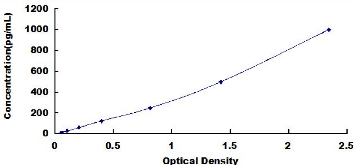
Typical Standard Curve for FGF18, Rat ELISA.
