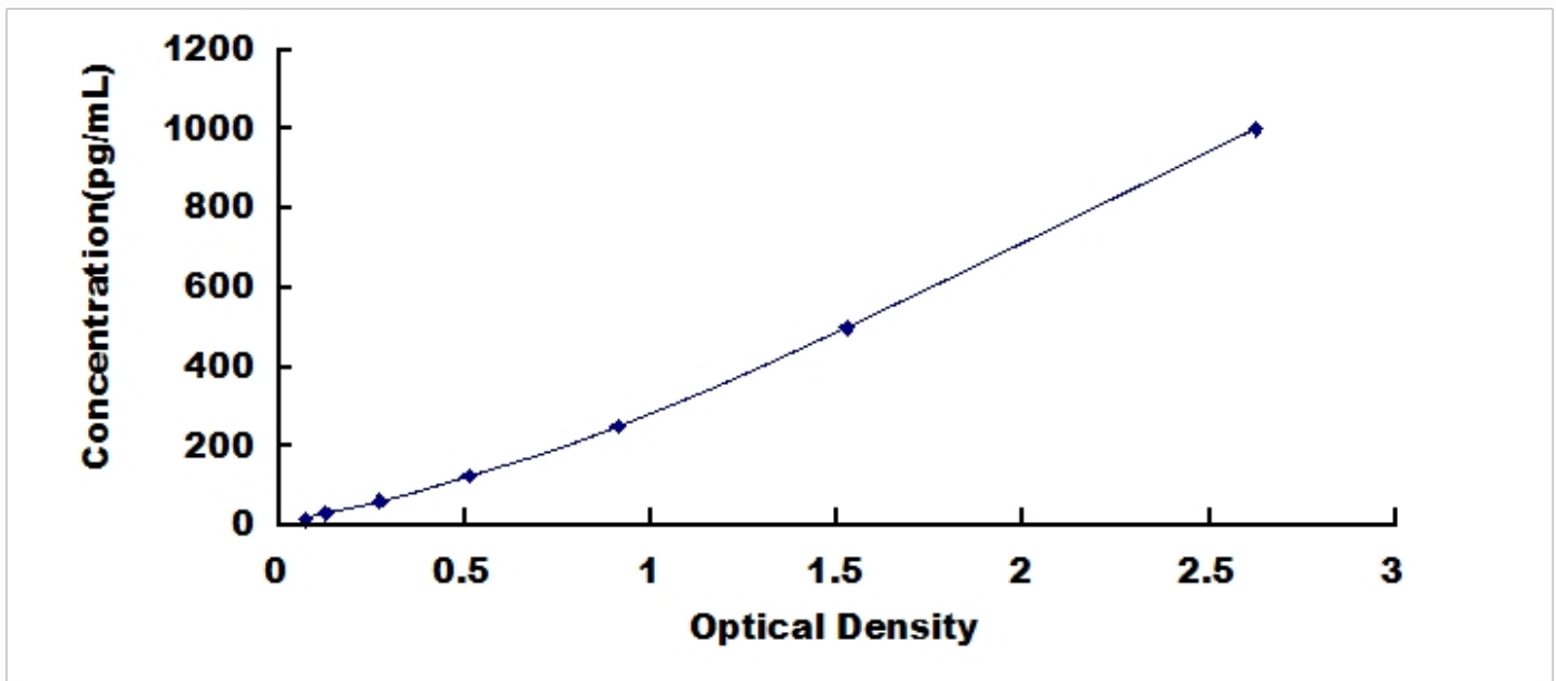
Typical Standard Curve for FGF3, Human ELISA.
