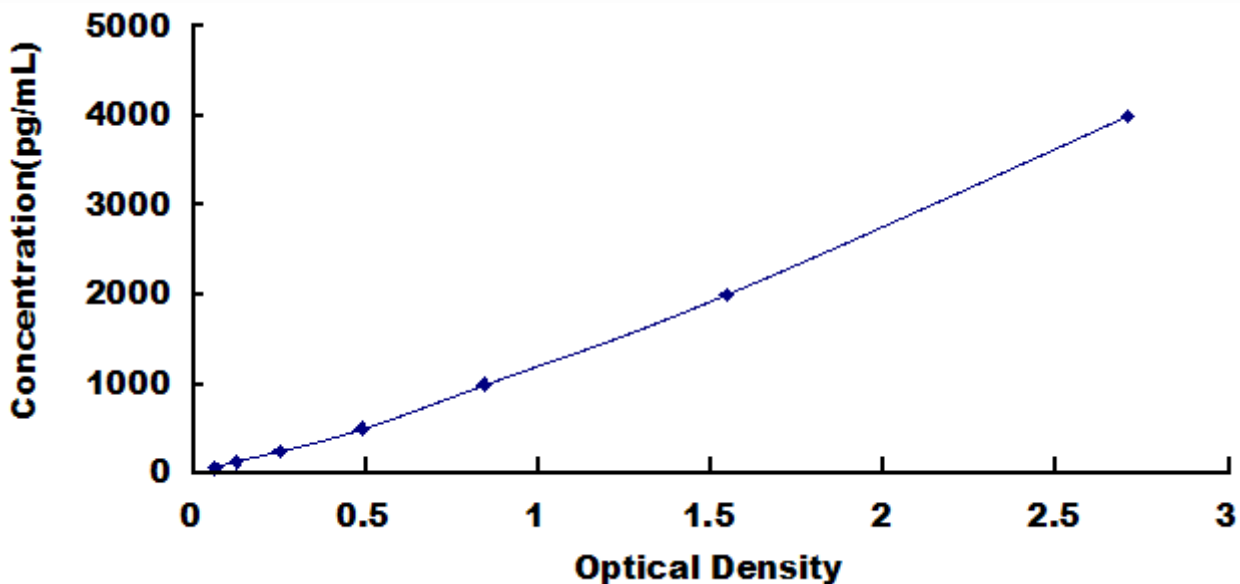
Typical Standard Curve for FGFR2, Human ELISA.
