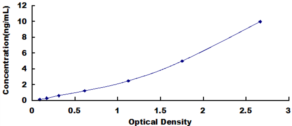
Typical Standard Curve for GRIA1, Human ELISA.
