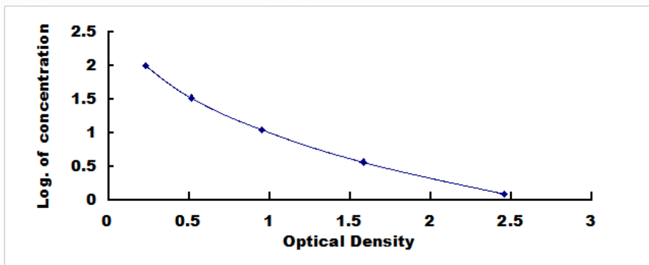
Typical Standard Curve for GSH ELISA.
