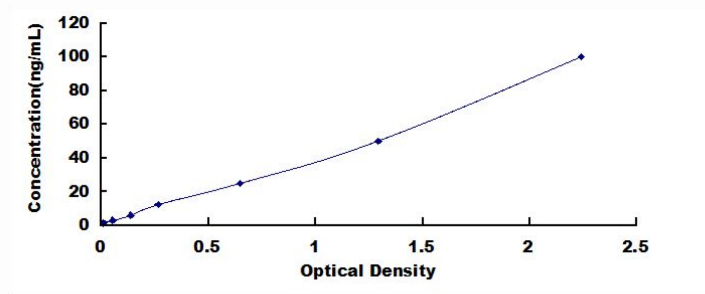
Typical Standard Curve for GPX4, Mouse ELISA.
