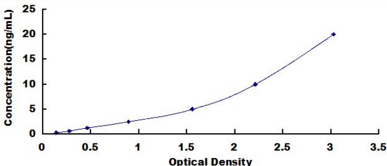
Typical Standard Curve for GP2, Rat ELISA.
