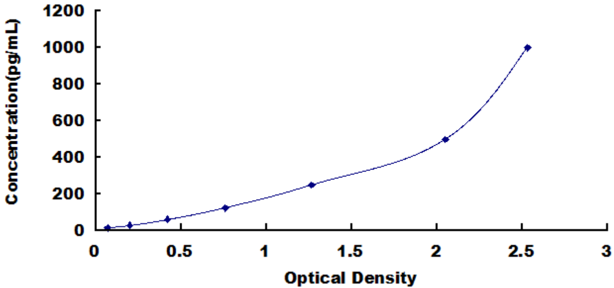
Typical Standard Curve for GREM1, Mouse ELISA.
