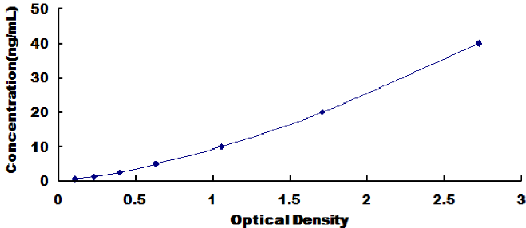
Typical Standard Curve for GADD45g, Mouse ELISA.
