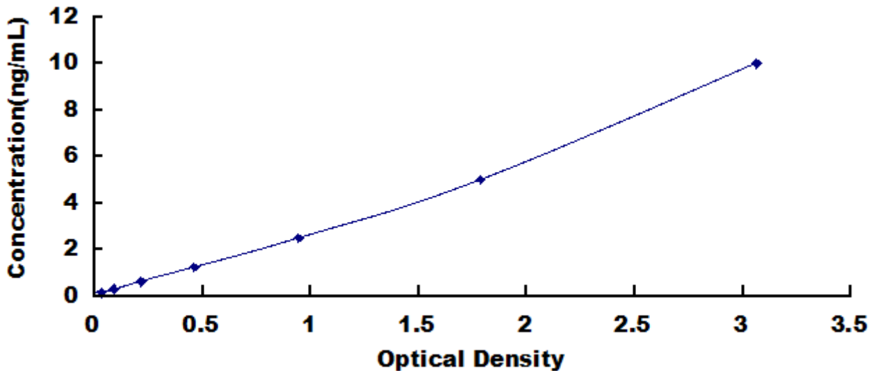
Typical Standard Curve for HPRT1, Mouse ELISA.
