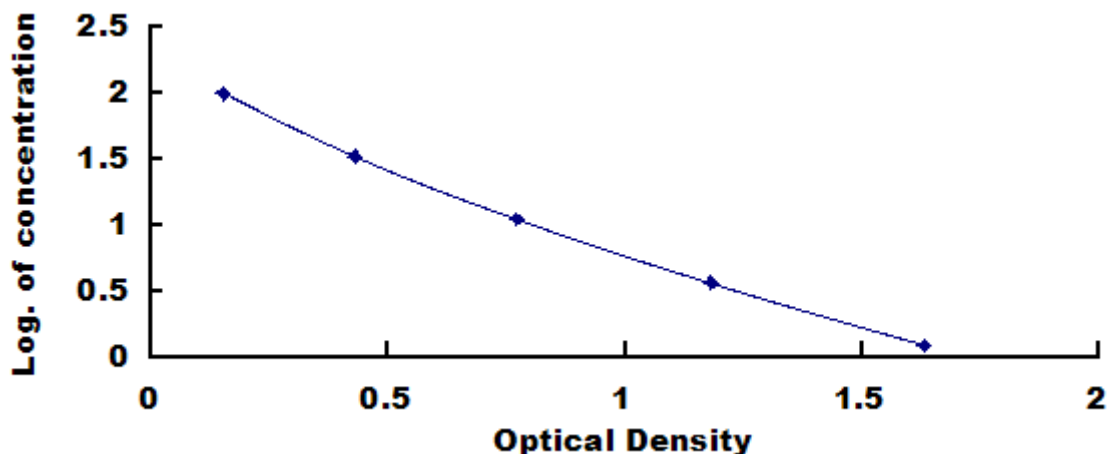
Typical Standard Curve for IgA, Gallus ELISA.
