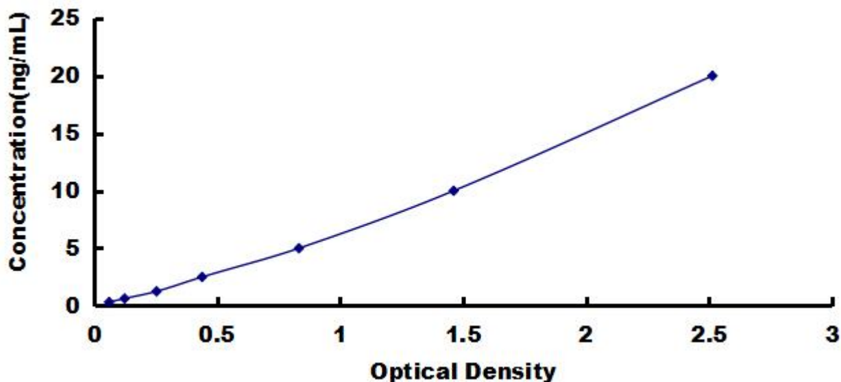
Typical Standard Curve for IgA, Human ELISA.
