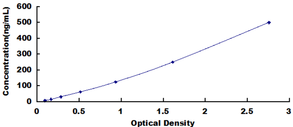
Typical Standard Curve for IgG, Ovine ELISA.
