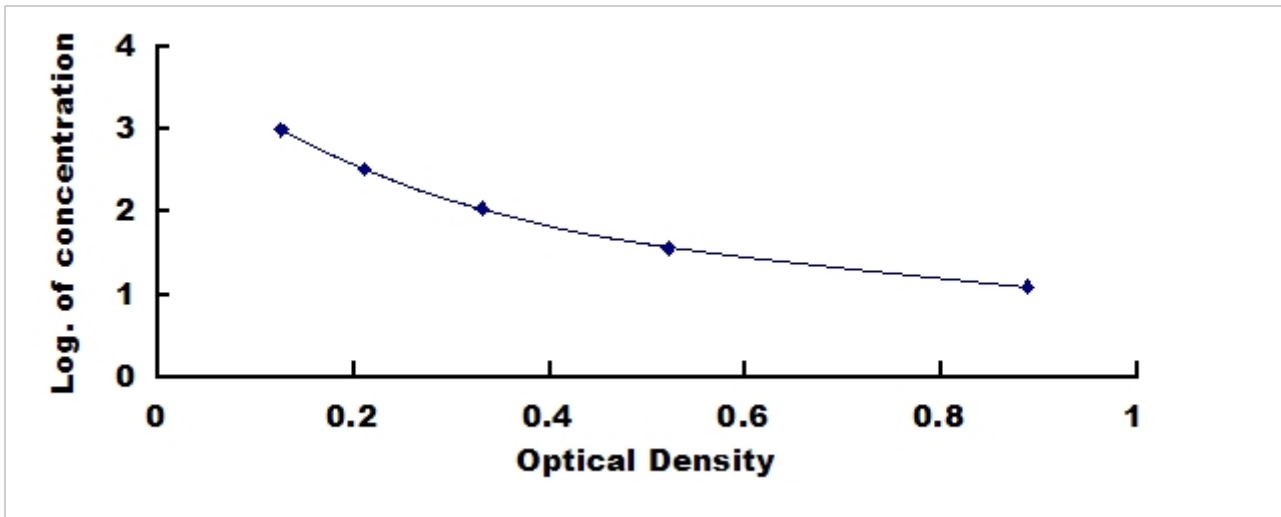
Typical Standard Curve for INHB, Rat ELISA.
