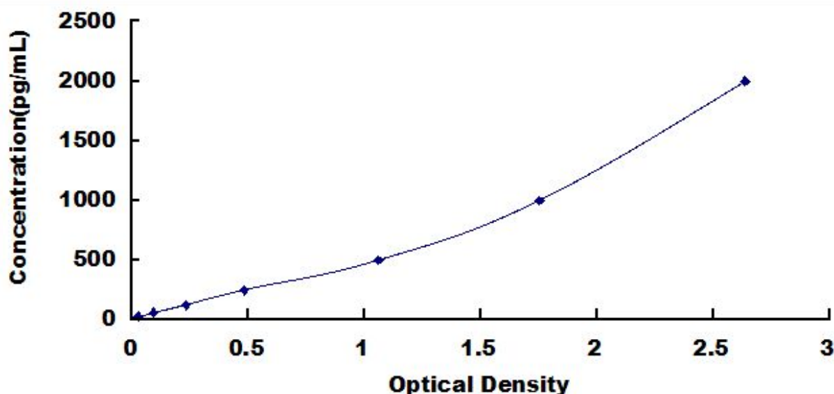
Typical Standard Curve for INHbC, Mouse ELISA.
