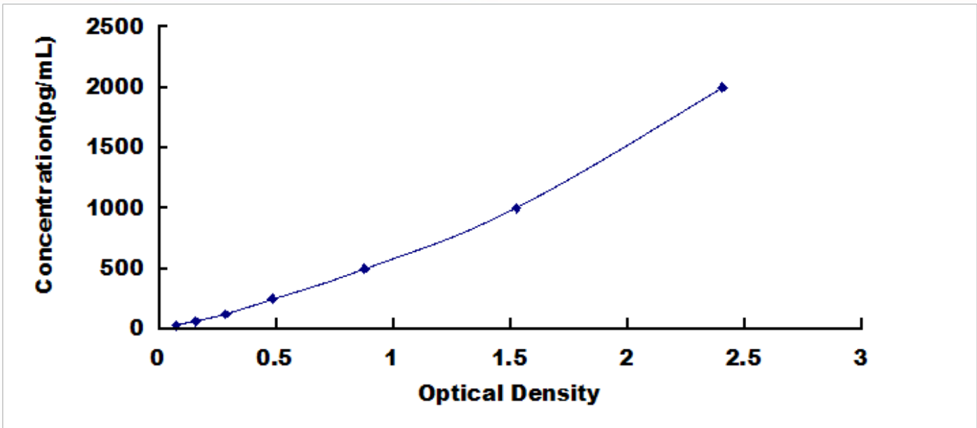
Typical Standard Curve for IL1RA, Mouse ELISA.
