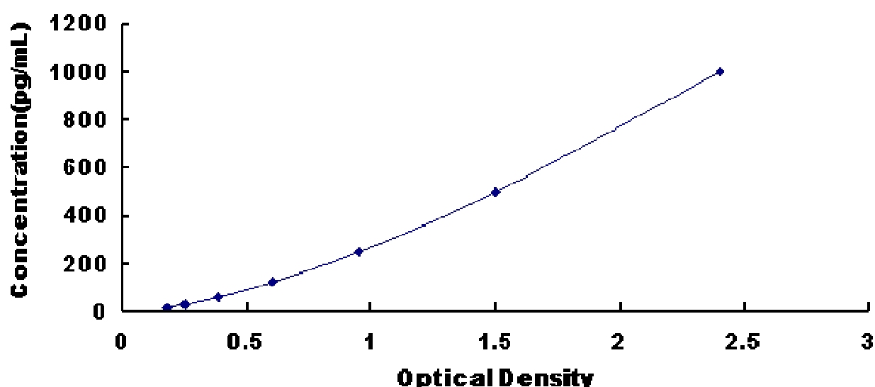
Typical Standard Curve for IL3, Rat ELISA.
