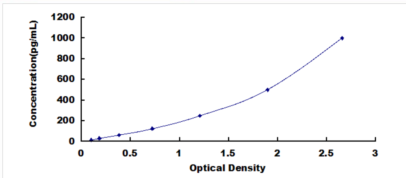
Typical Standard Curve for IL33, Human ELISA.
