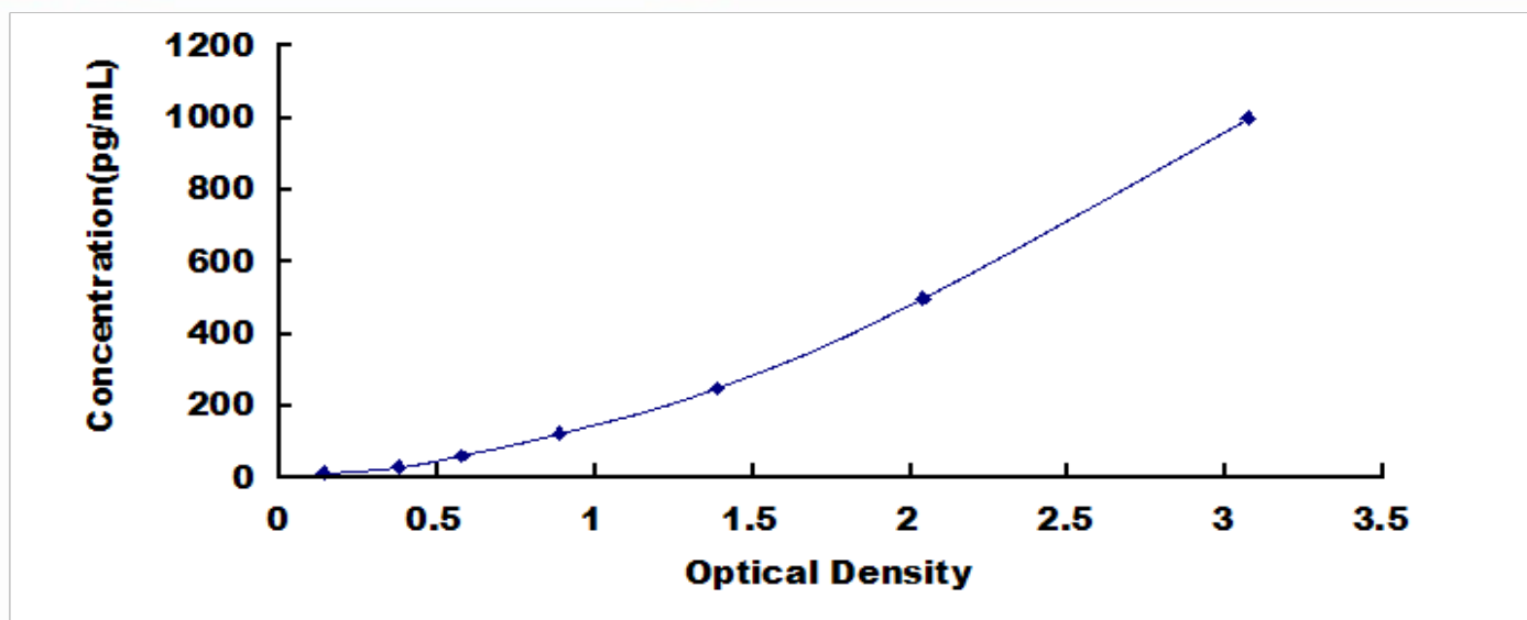
Typical Standard Curve for IL8, Rabbit ELISA.
