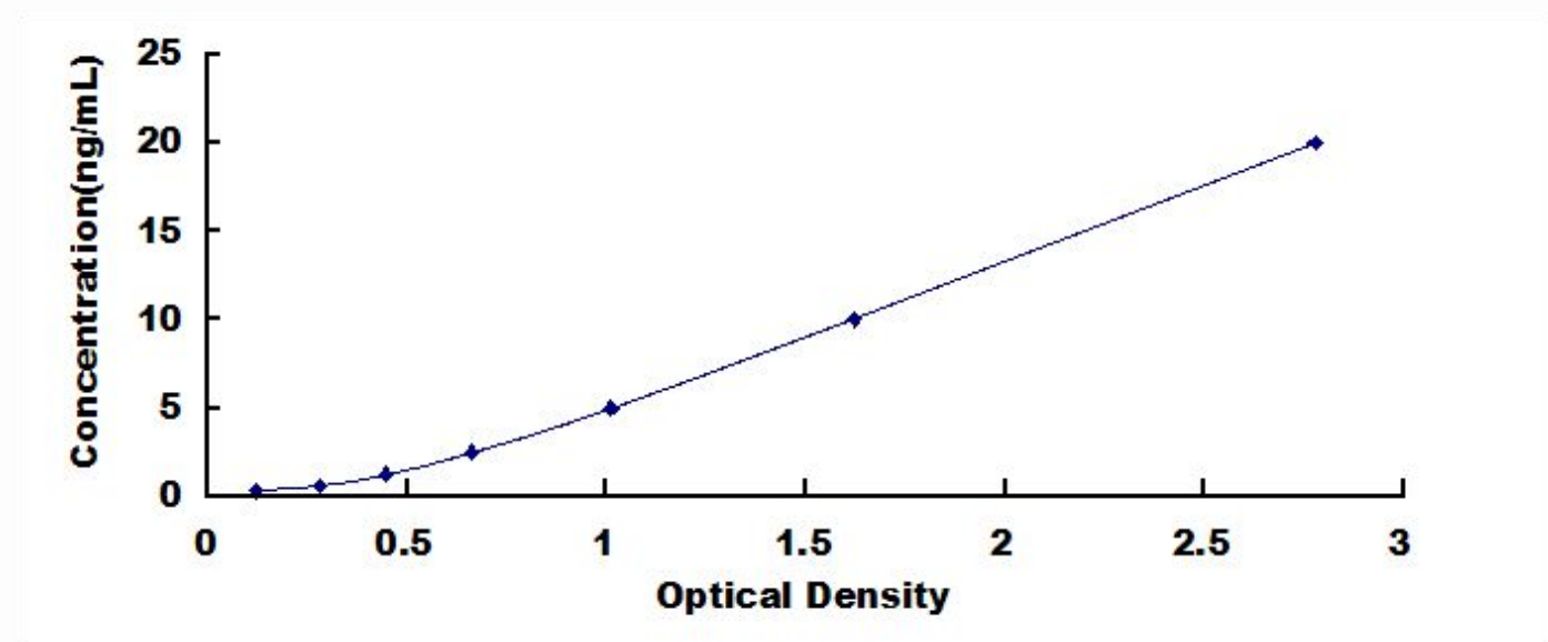
Typical Standard Curve for KLK4, Human ELISA.
