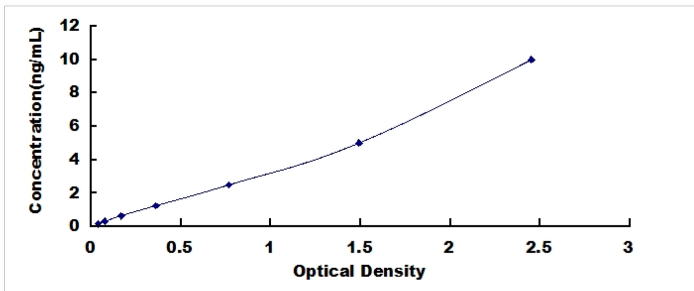
Typical Standard Curve for KRT9, Human ELISA.
