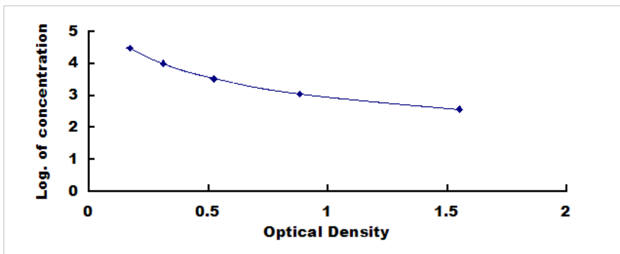
Typical Standard Curve for LH, Canine ELISA.
