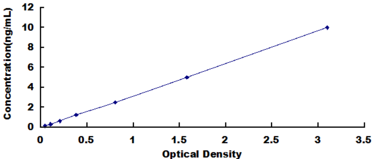
Typical Standard Curve for MICA, Human ELISA.
