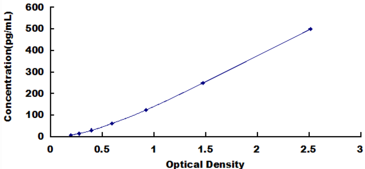
Typical Standard Curve for MIP1a, Canine ELISA.
