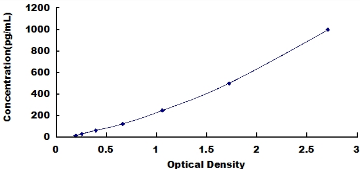
Typical Standard Curve for MMP14, Mouse ELISA.
