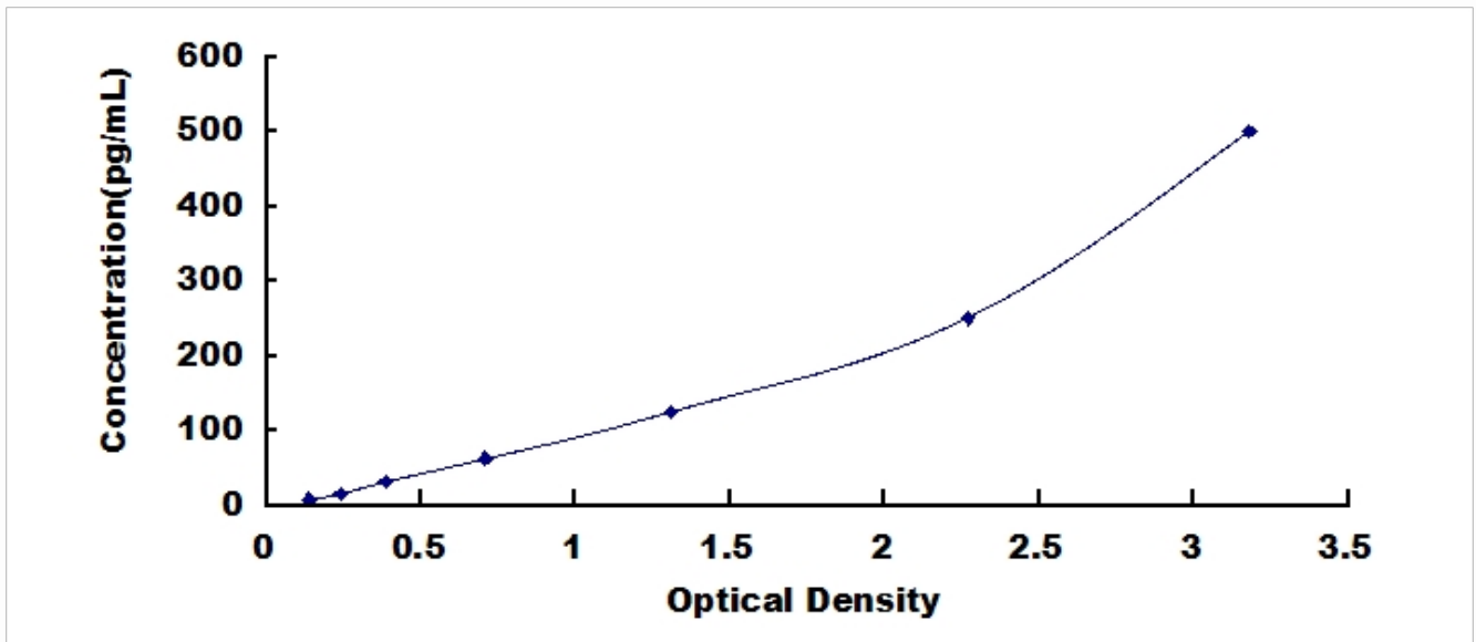
Typical Standard Curve for MYL2, Human ELISA.
