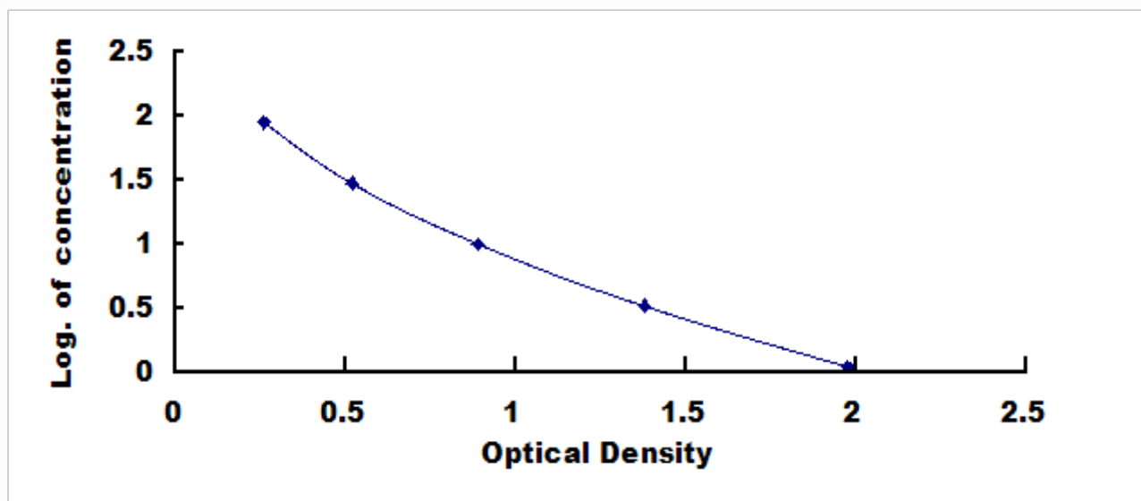
Typical Standard Curve for MSTN, Rat ELISA.
