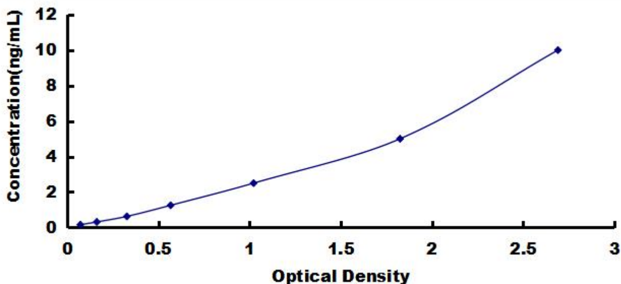
Typical Standard Curve for NOSIP, Human ELISA.
