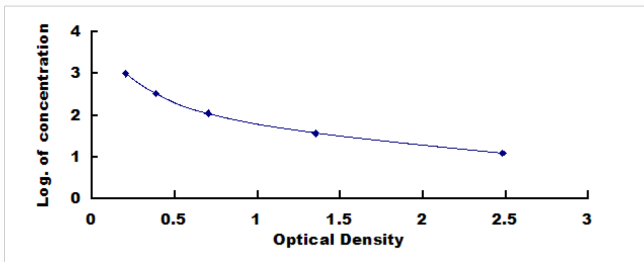
Typical Standard Curve for Oxytocin ELISA.
