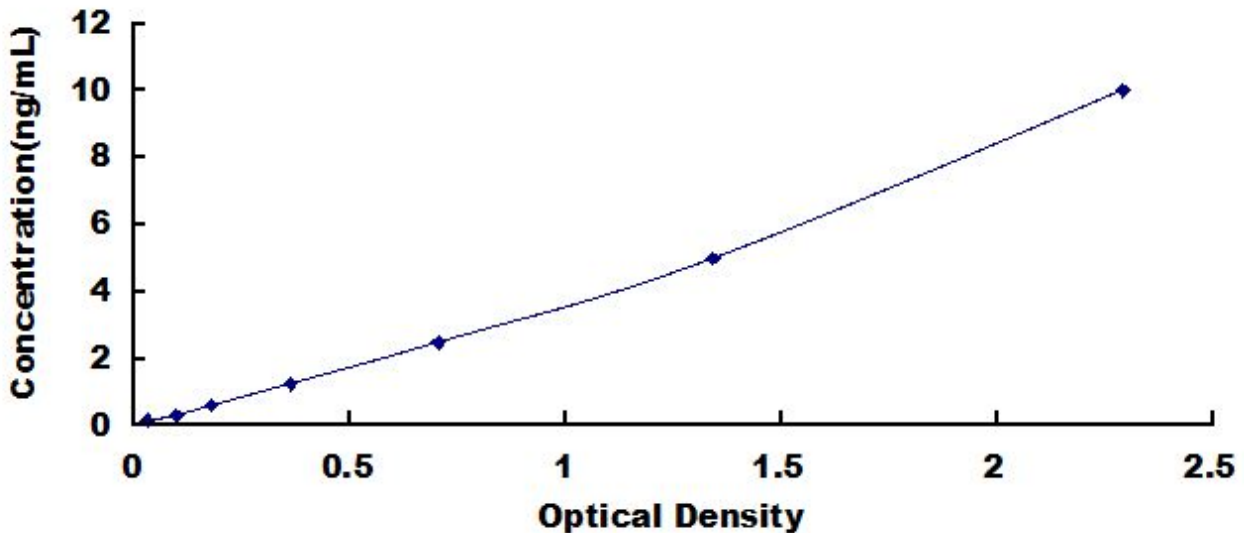
Typical Standard Curve for PEBP1, Mouse ELISA.
