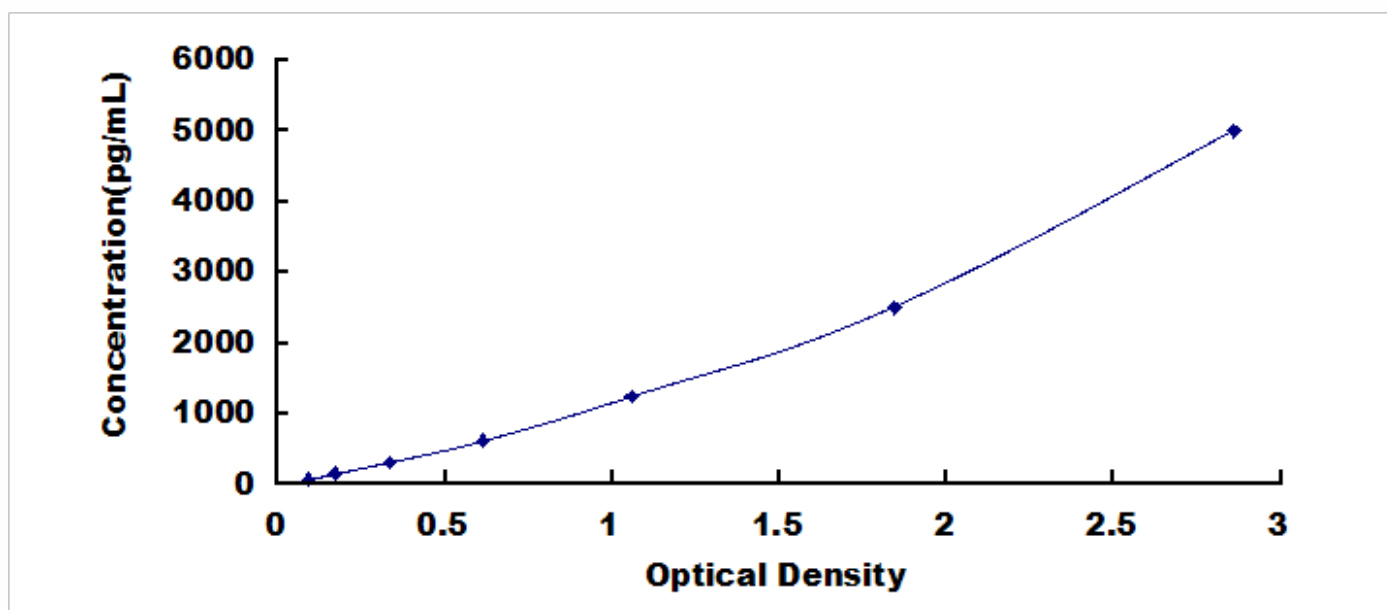
Typical Standard Curve for iPLA2, Human ELISA.
