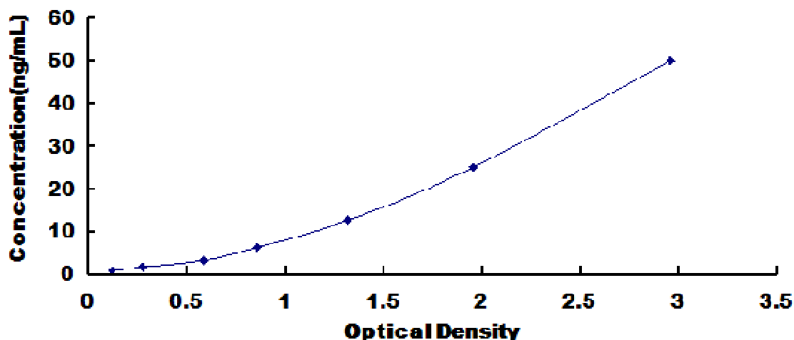
Typical Standard Curve for PIM1, Human ELISA.
