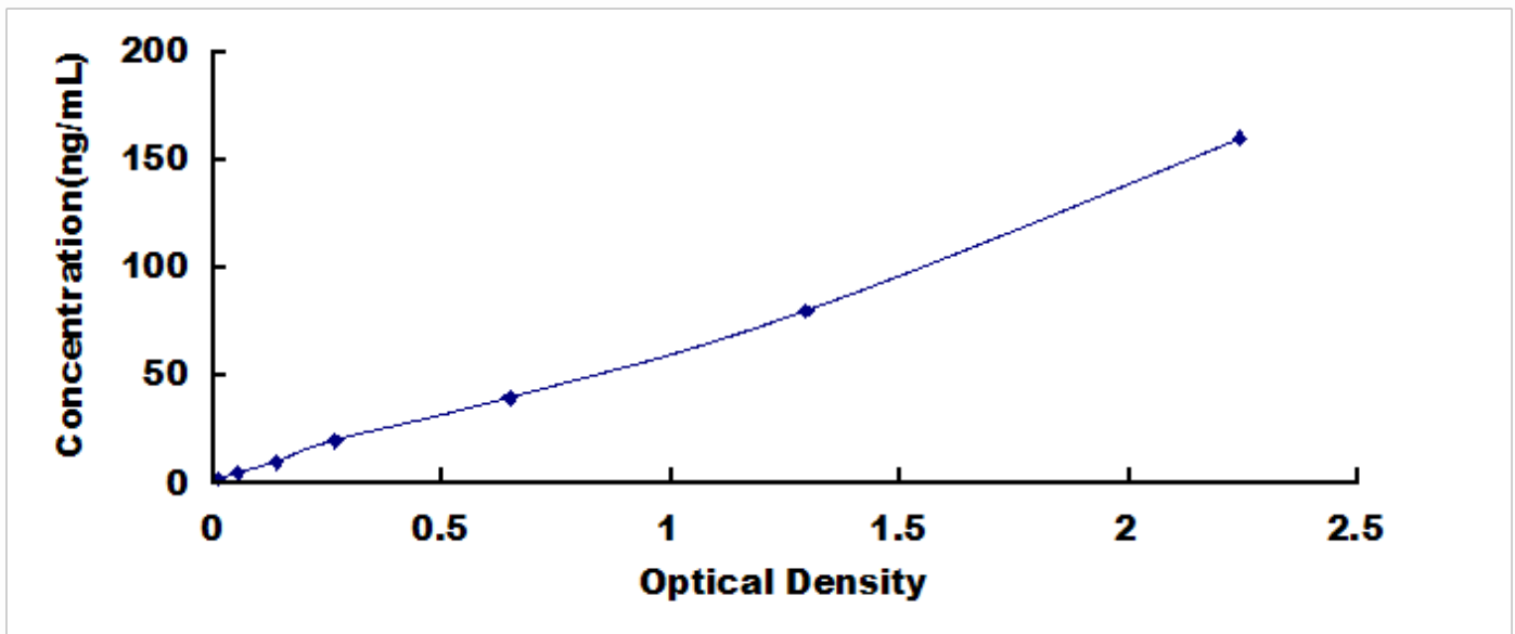
Typical Standard Curve for PCIII, Rat ELISA.
