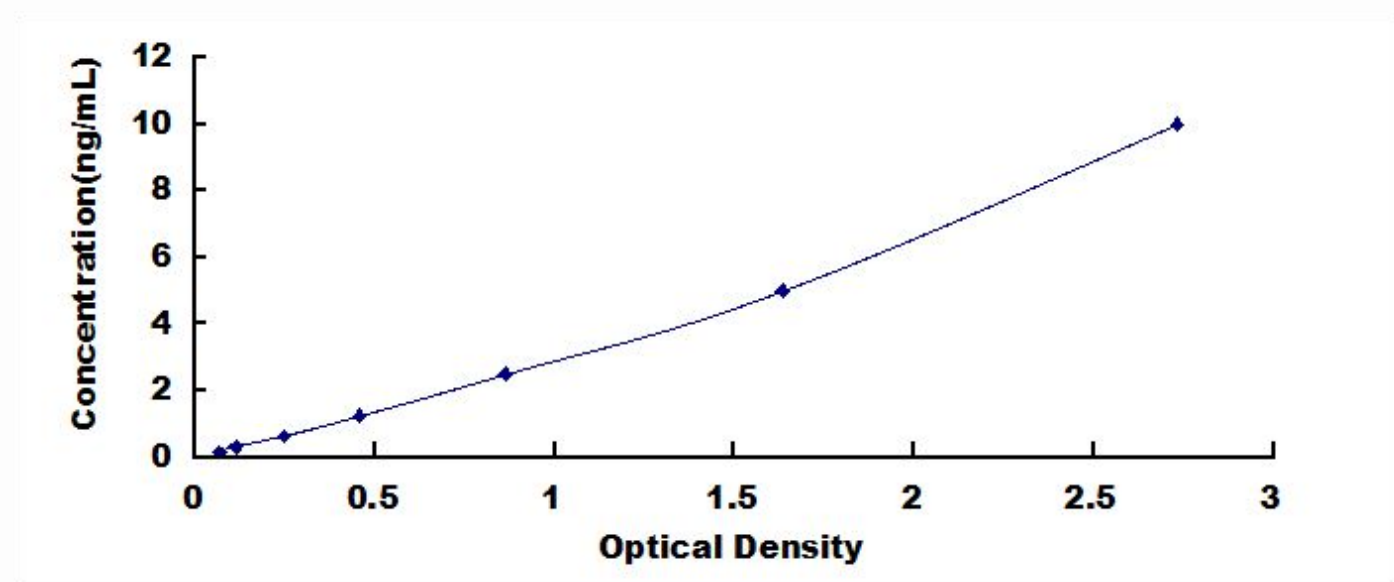
Typical Standard Curve for S100A11, Human ELISA.
