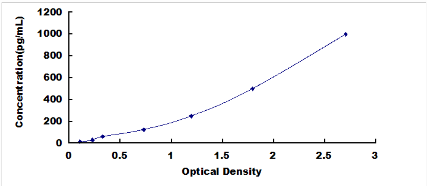
Typical Standard Curve for S100A9, Human ELISA.
