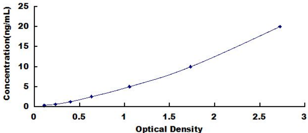
Typical Standard Curve for SIRT1, Mouse ELISA.
