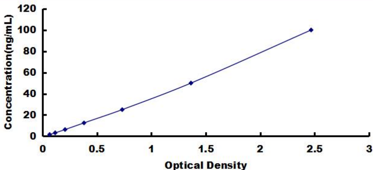
Typical Standard Curve for SLC7A9, Human ELISA.
