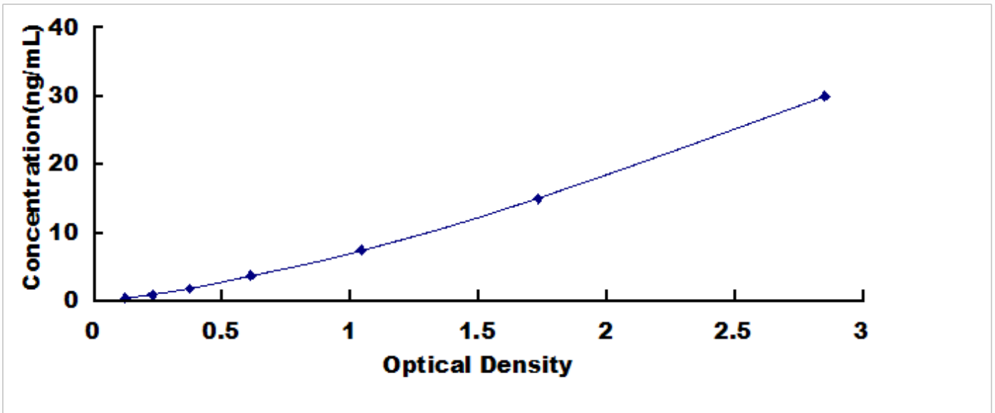
Typical Standard Curve for TIMP3, Equine ELISA.
