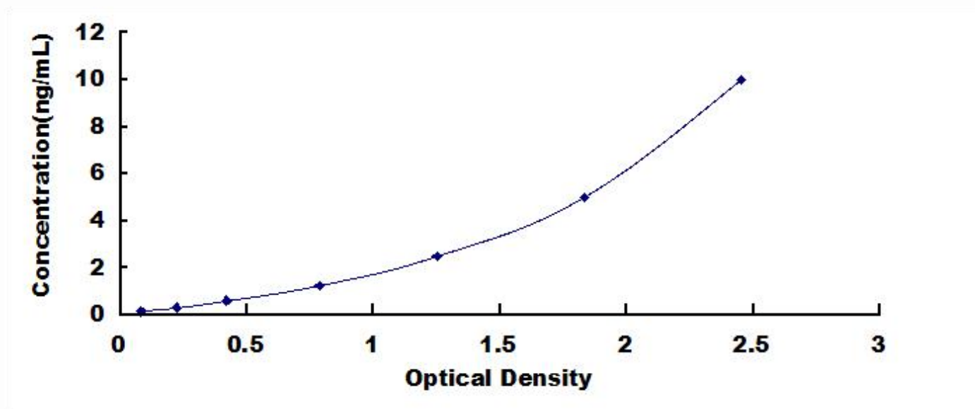
Typical Standard Curve for RELA, Human ELISA.
