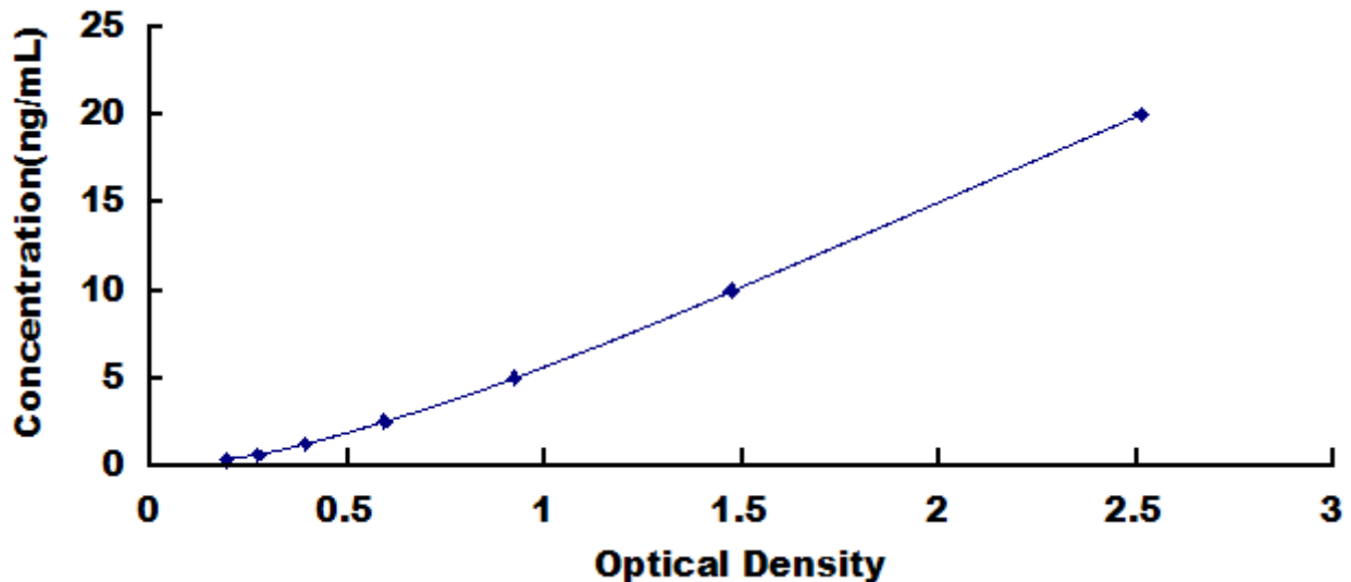
Typical Standard Curve for TGM1, Human ELISA.
