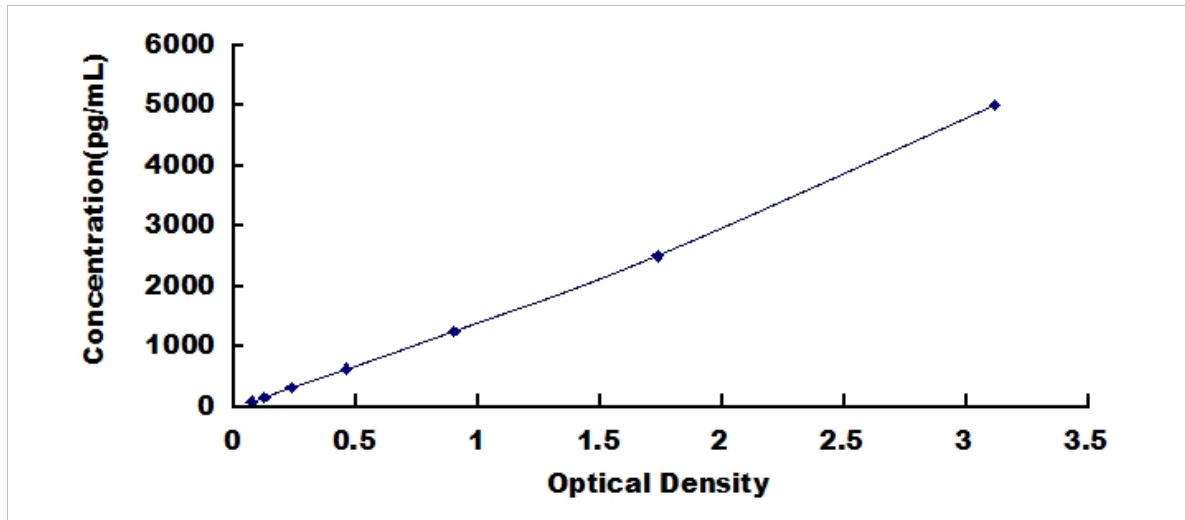
Typical Standard Curve for TP53, Rat ELISA.
