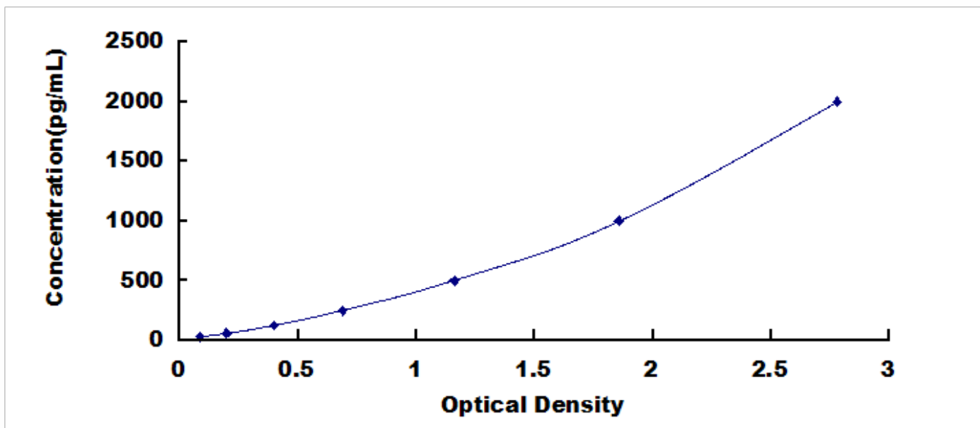
Typical Standard Curve for VDAC1, Human ELISA.
