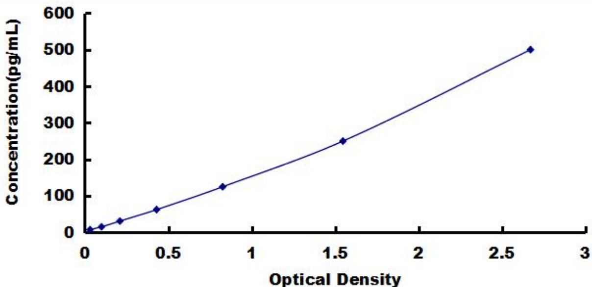
Typical Standard Curve for IL17, Canine ELISA.
