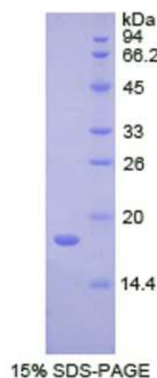
Human LCN6
