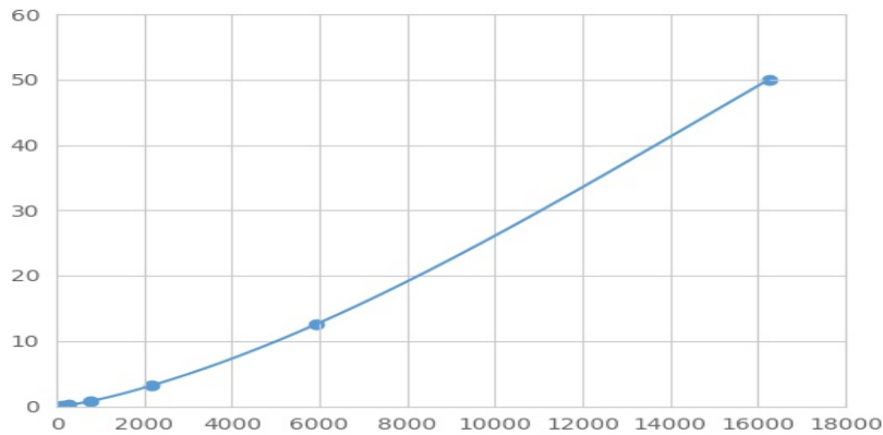
Typical Standard Curve for AANAT Magnetic Luminex Assay.
