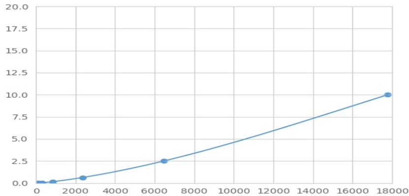
Typical Standard Curve for b3GAT1 Magnetic Luminex Assay.
