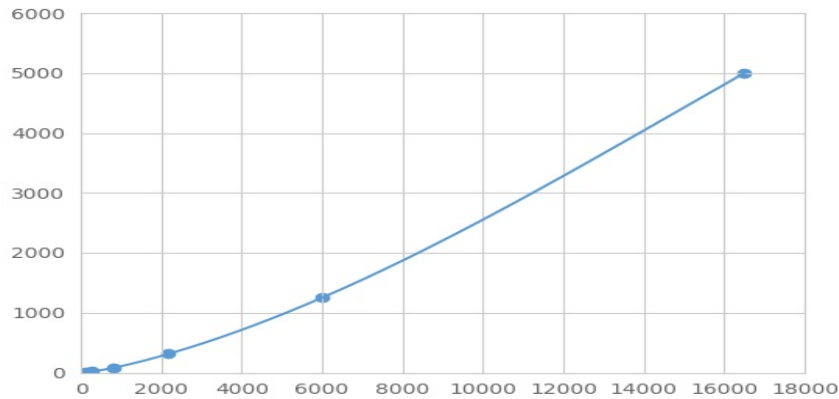
Typical Standard Curve for BCAN Magnetic Luminex Assay.
