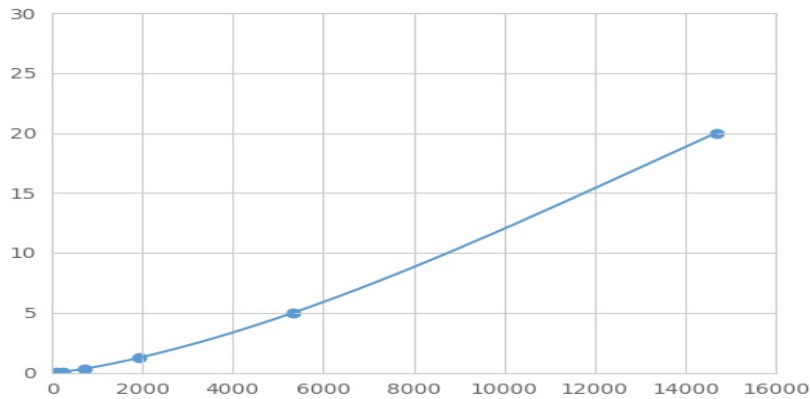
Typical Standard Curve for CYP2C19 Magnetic Luminex Assay.
