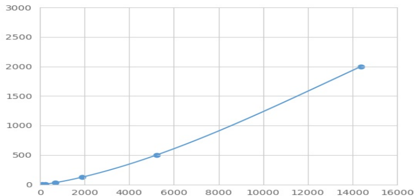
Typical Standard Curve for Hepc Magnetic Luminex Assay.
